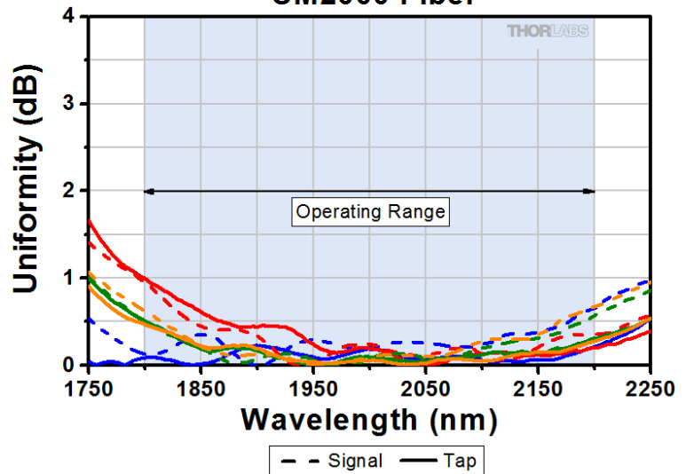
2000 nm Wideband Coupler, 50:50 Ratio, SM2000 Fiber
